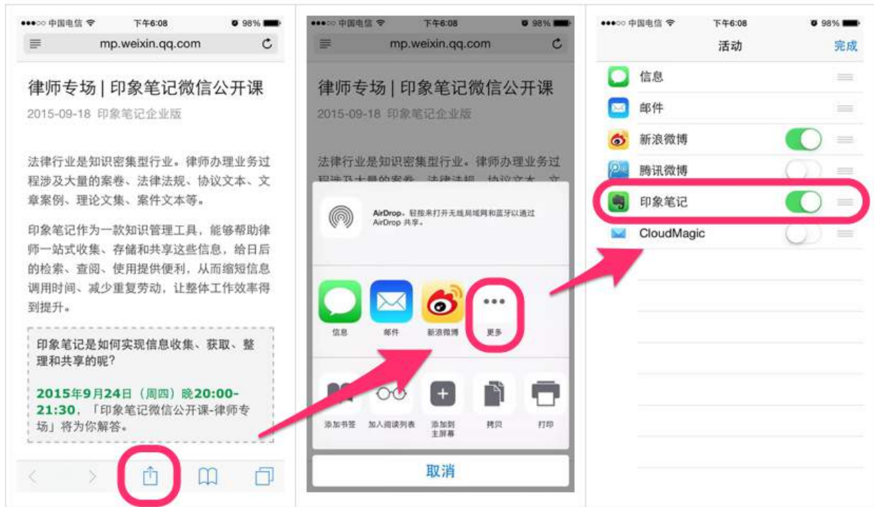
iOS Safari
